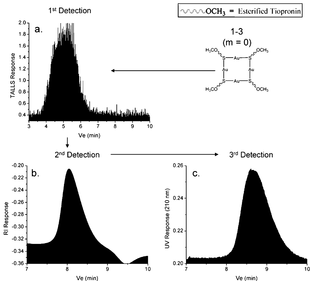
Figure 3. GPC chromatograms of gold(I)–thiolate precipitate (pre-MPC) dissolved in DMF (4 mg/mL). Tandem detection was performed through (a) triple angle laser light scattering, (b) refractive index, and (c) ultraviolet (210 nm) monitoring of the eluent. Lag-times between the chromatogram eluted volumes ( V_e ) are due to the tandem setup of the detectors.
