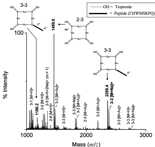
Figure 9. ESI-TOF mass spectrum (1000–3000 Da) of dialyzed (excess) peptide-substituted gold MPCs (2:1 MPC:peptide) doped with 50 \mu\text{L} of \text{H}_2\text{O} :ACN (1:1 and 1% glacial acetic acid).
